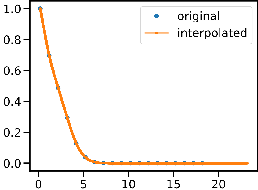
Overlap Interpolation After Training (14, 14, 0, 0)
